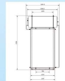
Installation Dimension
